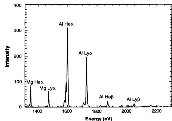
FIG. 15. Al-Mg alloy data from BJ5 (shot 3738) show a more consistent temperature (300–350 eV) between Al and Mg, indicating a uniform mix, as one would expect with an alloy.
