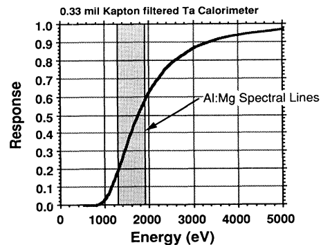
FIG. 6. Relative detector responses versus photon energy for our filtered copper XRDs and tantalum calorimeters.
