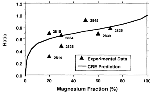
FIG. 10. Measured ratio of the magnesium line energy to the total line energy versus magnesium fraction.
