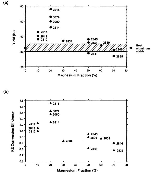
FIG. 7. Measured kilovolt x-ray yield from the wire arrays described in Table I. The (a) measured yields are also normalized to the implosion kinetic energy in (b).
